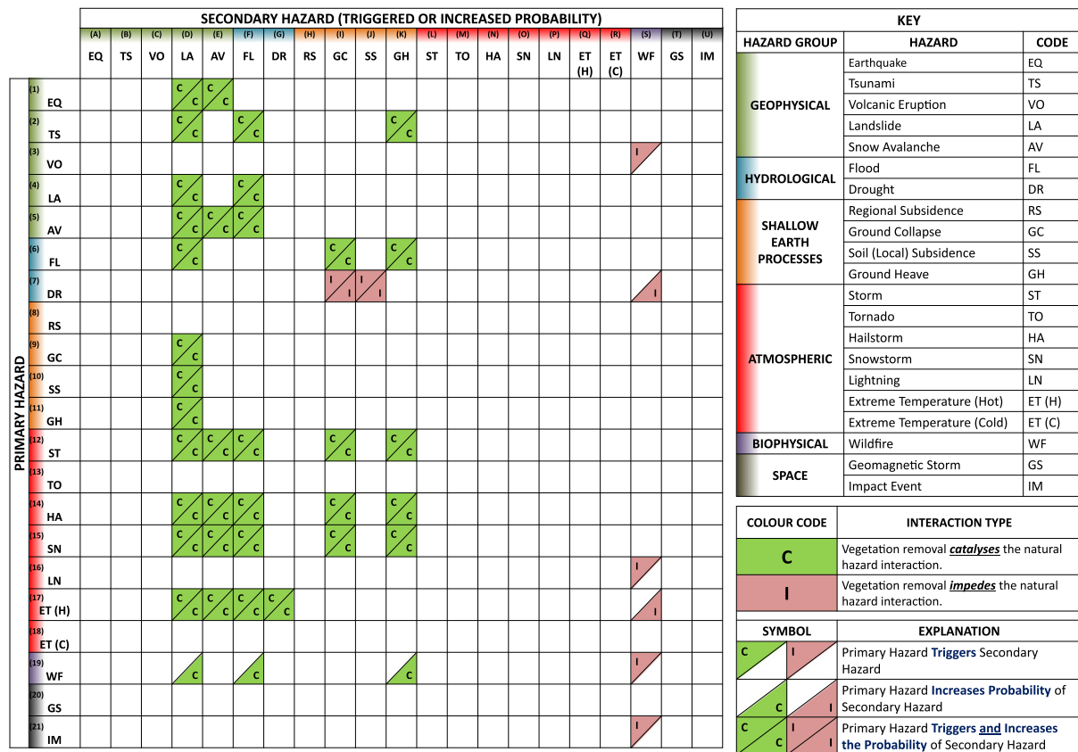
Fig. 8. Influence of vegetation removal on natural hazard interactions. A 21 × 21 interaction matrix with primary hazards on the vertical axis and secondary hazards on the horizontal axis. These hazards are coded and classified as explained in the key and Table 4. This interaction matrix shows cases where a primary hazard could trigger a secondary hazard (upper-left triangle shaded) and cases where a primary hazard could increase the probability of a secondary hazard being triggered (bottom-right triangle shaded). Where both triangles are shaded, this indicates that the primary hazard could both trigger and increase the probability of a secondary hazard. Where vegetation removal is noted to catalyse the given hazard interaction the cell is shaded green and labelled with a 'C'. Where vegetation removal is noted to impede the given hazard interaction the cell is shaded pink and labelled with an 'I'.
