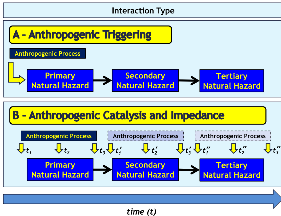
Fig. 4. Mechanisms relating anthropogenic process types to natural hazards and natural hazard interactions. Two mechanisms are presented by which anthropogenic processes, such as those outlined in Table 2 , may relate to natural hazards, such as those outlined in Table 4 . The first mechanism (A) is anthropogenic triggering, where an anthropogenic process may trigger a primary natural hazard. This in turn may trigger further natural hazards to form a network of interactions (cascade). The second mechanism (B) is anthropogenic catalysis and impedance, where an anthropogenic process may catalyse or impede a defined primary natural hazard triggering a secondary natural hazard interaction. The anthropogenic process could occur before ( t_1 ), during ( t_2 ) or after ( t_3 ) the primary natural hazard, and at any point in a cascade system ( t' and t'' ).
