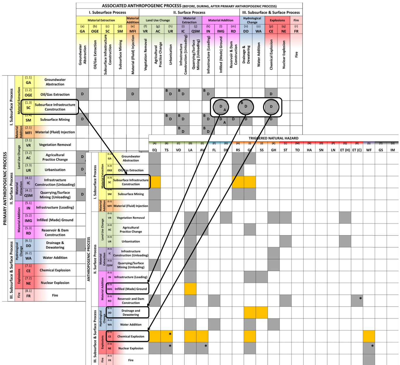
Fig. 10. Triggering of natural hazards by an ensemble of anthropogenic processes, visualised by combining Figs. 1 and 5. A figure combining the 18 × 18 interaction matrix of anthropogenic process type interactions, with interactions indicated using grey cell shading (Fig. 1) with the 18 × 21 interaction matrix of anthropogenic process types triggering natural hazards, with interactions indicated using grey and orange cell shading (Fig. 5). Full details of each interaction matrix can be found in the respective figures. (i) (underlying matrix) An example of a primary anthropogenic process, subsurface infrastructure construction (SC), that may trigger three associated secondary anthropogenic processes (shaded in grey and circled): infilled (made) ground (IMG), drainage and dewatering (DD) and chemical explosions (CE). (ii) (overlying matrix) Together this ensemble of four anthropogenic processes could trigger up to eight different natural hazards (shaded in orange): earthquakes (EQ), tsunamis (TS), landslides (LA), avalanches (AV), regional subsidence (RS), ground collapse (GC), soil subsidence (SS) and wildfires (WF). Other anthropogenic process-natural hazard interactions are shown in grey. The natural hazards triggered in any given region will depend on many process-specific and location-specific factors. For example, the detonation of chemical explosives for blasting, used in subsurface infrastructure construction, is unlikely to be connected to the triggering of tsunamis.
