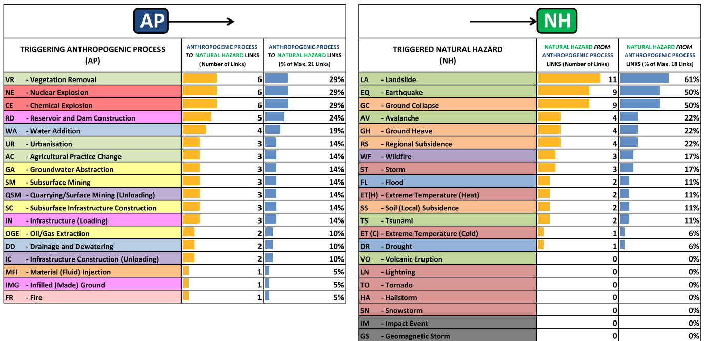
Fig. 6. Ranking of individual anthropogenic processes (AP) and natural hazards (NH) based on the total number and percentage of the maximum possible (left) AP to NH links and (right) NH from AP links. Using the interaction matrix (Fig. 5), the number of anthropogenic process natural hazard links is summed for each anthropogenic process in this study, and then ranked (left). This was then repeated for each natural hazard, summing and ranking triggered natural hazard from anthropogenic process links (right). For both we also present the results as a percentage of the maximum possible number of links (21 anthropogenic process to triggering natural hazard links; 18 natural hazards triggered by anthropogenic process links). Figure compiled using information from Fig. 5.
