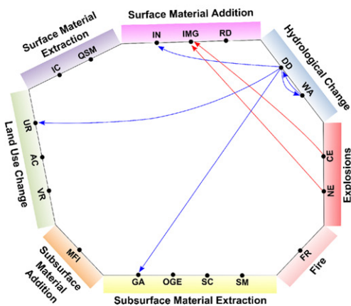
Fig. 2. Network linkage diagrams showing interactions between 18 anthropogenic process types, based on a design-structure presented in Gill and Malamud (2014). The principal octagon network linkage diagram (A) features 18 coded anthropogenic process types, with codes noted in the key (see also Table 2), and is an alternative visualisation of information presented in Fig. 1. Individual octagon network linkage diagrams (B) are also included for the three different groups: (I) subsurface, (II) surface and (III) both (subsurface and surface). In all octagon network linkage diagrams, anthropogenic process sub-groups follow the same colour coding as introduced in Table 2. Arrows are used to show where a primary anthropogenic process type may trigger an associated secondary anthropogenic process type to occur. Lines are coloured according to the sub-group in which the relationship is initiated. The primary anthropogenic process type may trigger the associated secondary anthropogenic process type before, simultaneously with, or after the primary anthropogenic process type. Although not included in this figure, in some cases it is possible that one anthropogenic process type may trigger further (or more intense) occurrences of itself.
