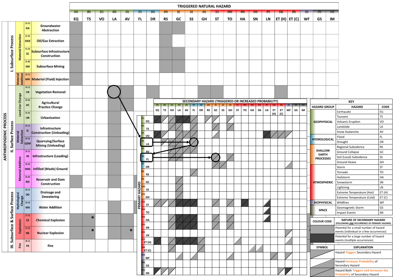
Fig. 9. Initiation of network of interactions (cascade) visualised by combining Figs. 5 and 7. A figure combining the 18 × 21 interaction matrix of anthropogenic process types triggering natural hazards (Fig. 5) with the 21 × 21 interaction matrix of natural hazards triggering natural hazards (Fig. 7). Full details of each interaction matrix can be found in the respective figures. An example of a network of interactions (cascade) is visualised. In this example, vegetation removal (VR) is shown to trigger a landslide (LA), which then triggers a flood (FL), which then triggers ground collapse (GC).
